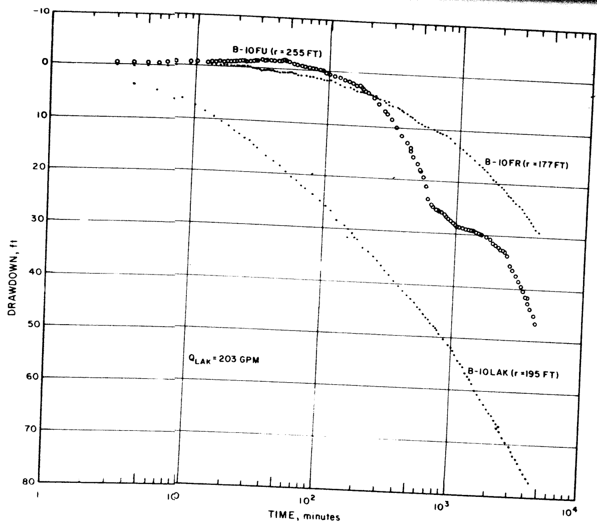
Figure 8 : Semilogarithmic Graphs of Drawdown for B-IO Observation Well Group, Lakota Aquifer Test
