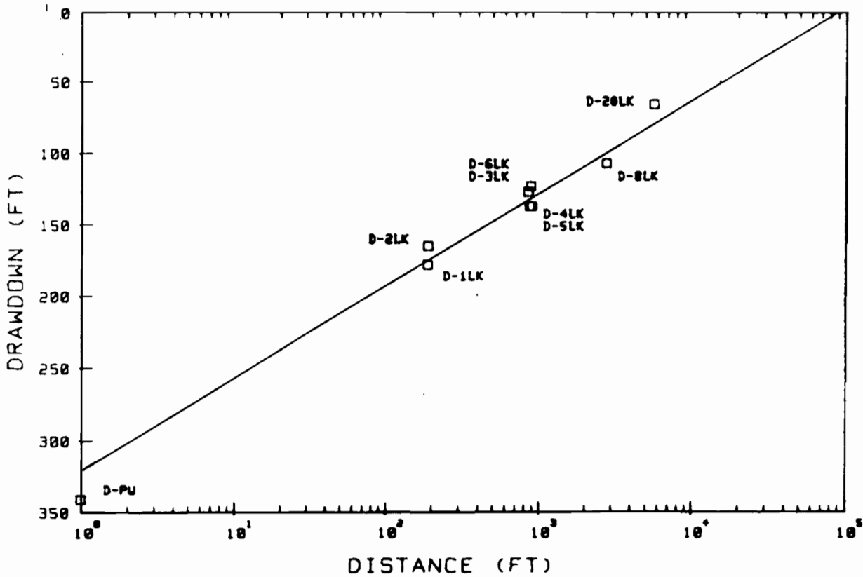
FIGURE 3. DISTANCE-DRAWDOWN GRAPH
