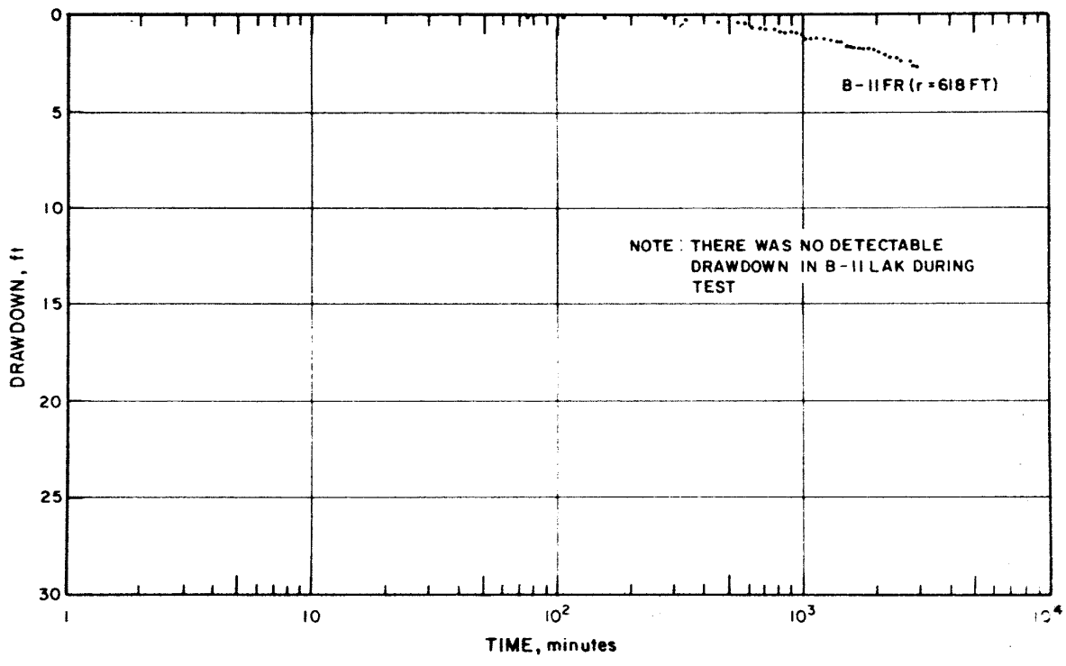
Figure 29: Semilogarithmic Graph of Drawdown for B-II Observation Well Group, Fall River Aquifer Test
