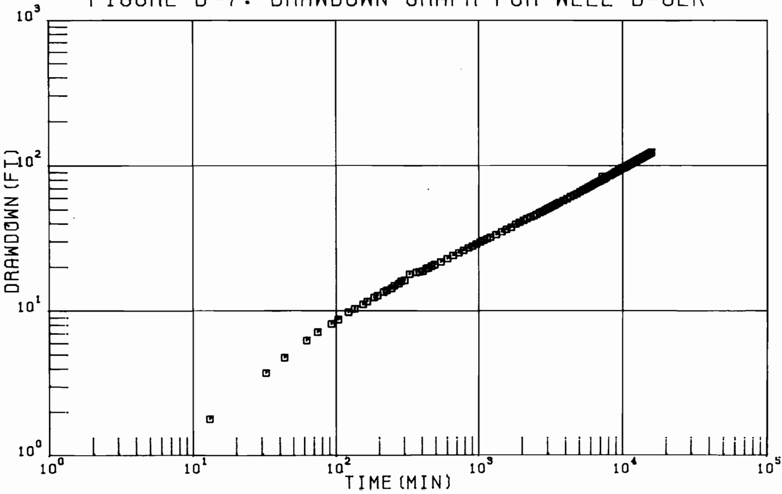
FIGURE B-7: DRAWDOWN GRAPH FOR WELL D-6LK
