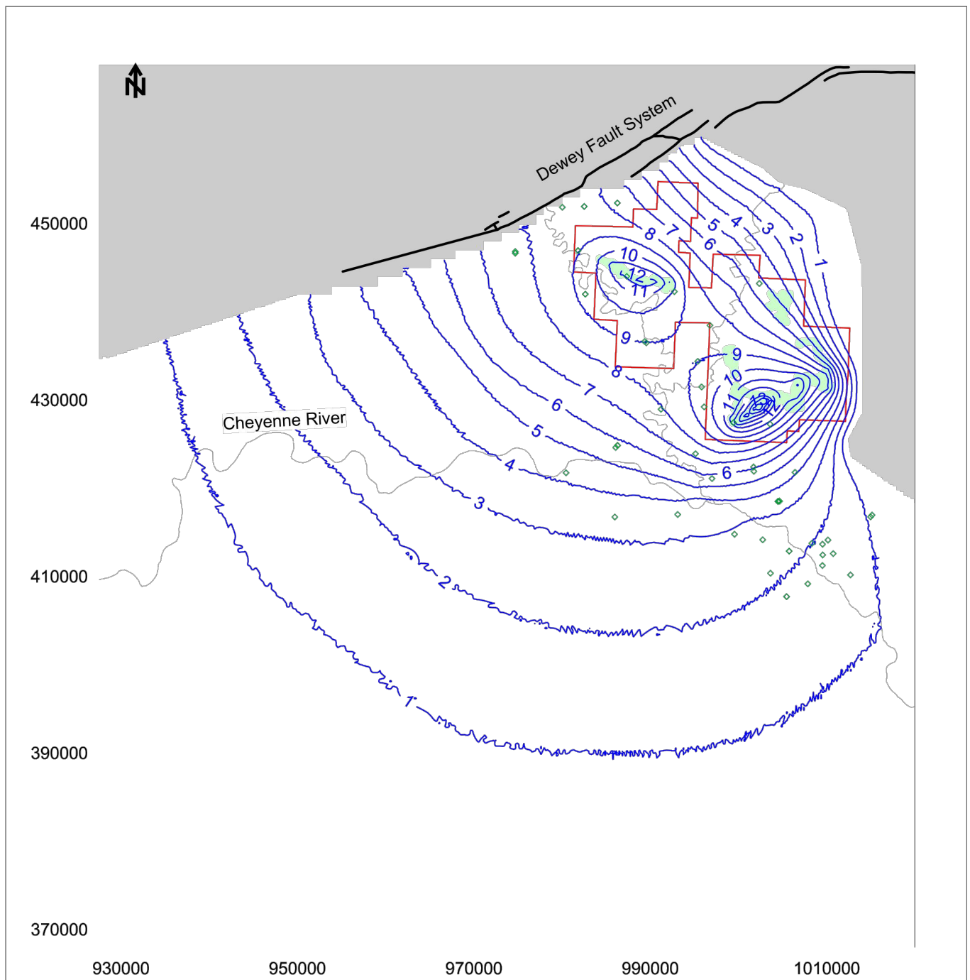
Drawdown at End of Stress Period 8
